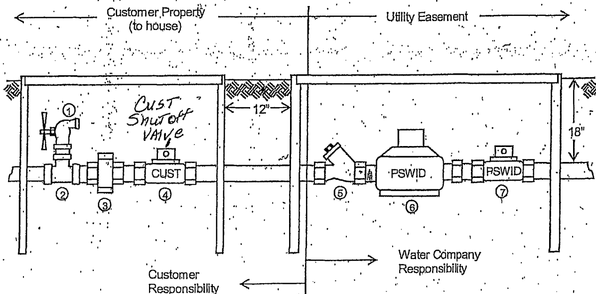
DIAGRAM FOR REQUIRED CUSTOMER SIDE CONNECTION TO METER
